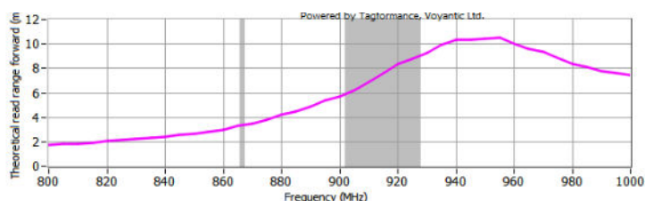
Read Range
